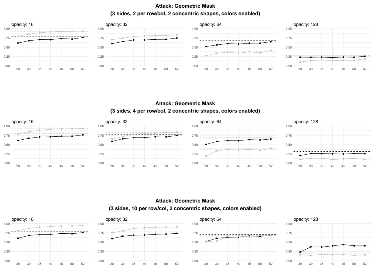
Figure 3.8: Evaluating the most effective masks on CIFAR10. The X-axis shows intermediary layers, the Y-axis shows accuracy, the black line indicates natural training, dotted horizontal lines show ensemble performance.
