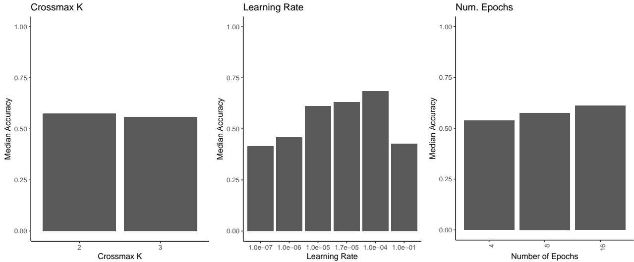
Figure 3.1: Hyperparameter search on the reproduced architecture.
