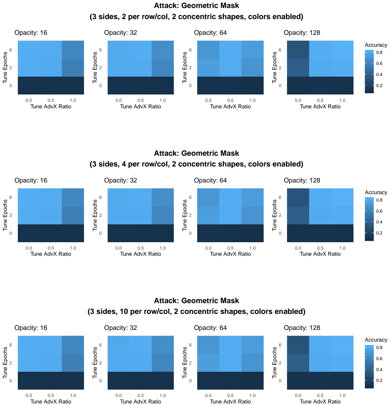
Figure 3.9: Evaluating the most effective masks on the Backbone. The X-axis shows the ratio of perturbed masks in the tuning set, the Y-axis shows the number of epochs the model was tuned with.
