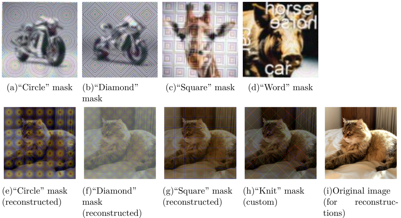
Figure 2.3: Selected examples by hCAPTCHA and their optimized reconstructions. The “Word” overlay was omitted and replaced with a custom “Knit” mask.
