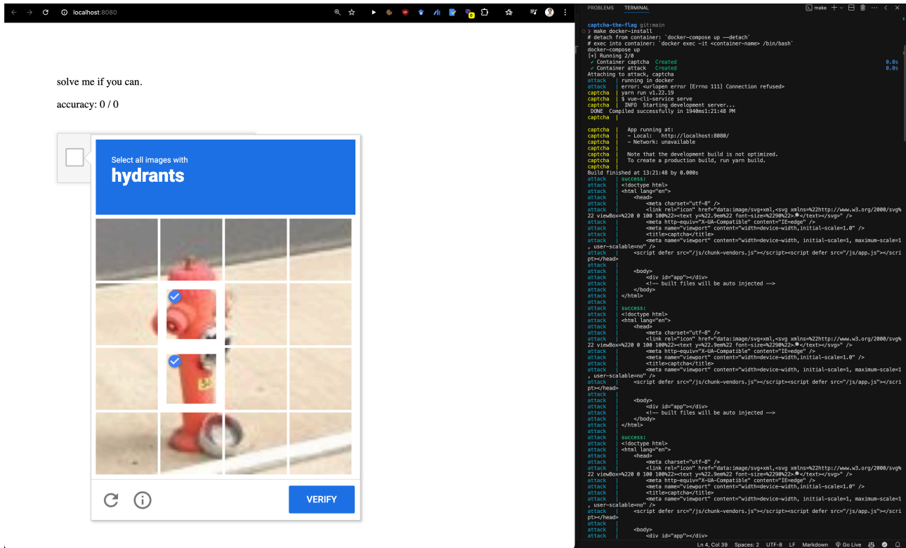
Figure 2.1: ReCAPTCHAv2 cybersecurity emulation framework https://github.com/ETH-DISCO/captcha-the-flag
