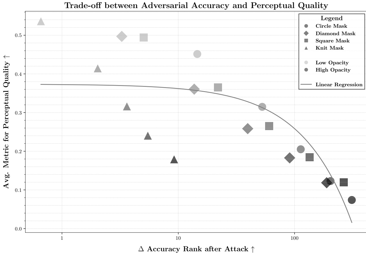
Figure 2.8: Accuracy vs. Perceptual Quality Trade-off
