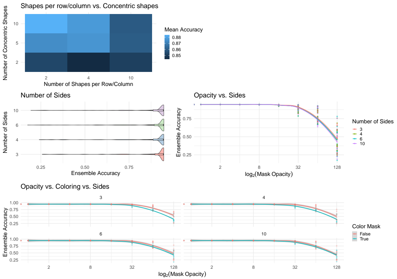
Figure 3.5: Limiting mask parameters to the most effective ones for CIFAR10. The lower most plot encodes the opacity in the x-axis, the better performing ensemble accuracy in the y-axis, the number of sides in the individual subplots and whether masks are colored or not as the color.
