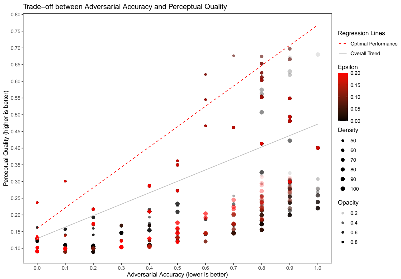
Figure 2.7: Accuracy-perceptibility trade-off: We compare the strength of a diamond mask with different opacities, densities and FGSM perturbation settings against their perceptibility based on our proxy metric.
