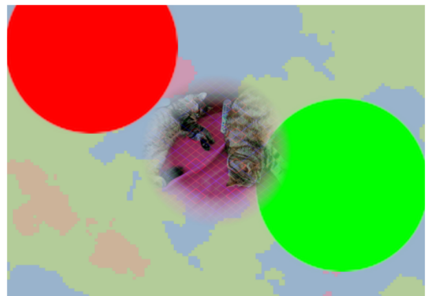
Figure 2.5: Reconstruction (arbitrary parameters).
