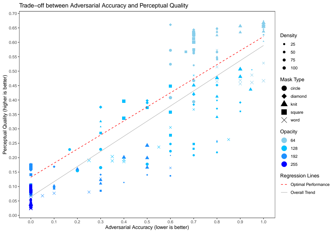
Figure 2.6: Accuracy-perceptibility trade-off: We compare the strength of all our masks with different opacities and densities against their perceptibility based on our proxy metric.
